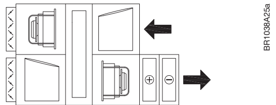
Counter flow heat exchanger AHU
