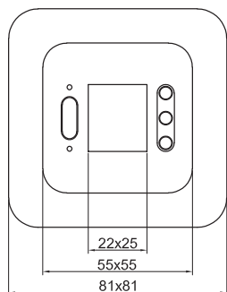
Dimensions (mm)
