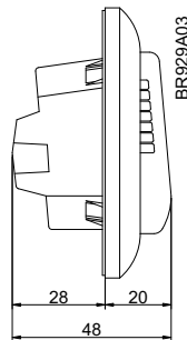
Dimensions (mm)
