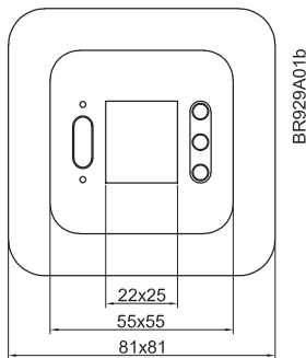
Dimensions (mm)
