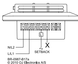
Night setback
