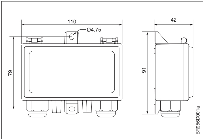
Fig. 1 - Dimensioned drawing
