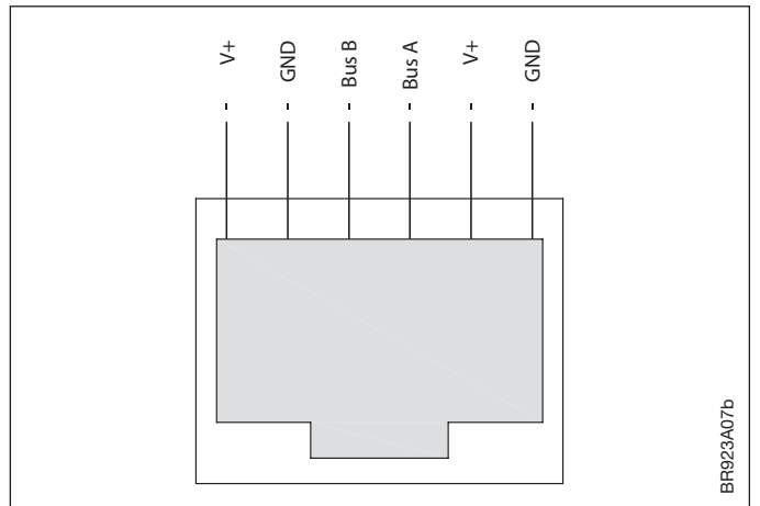
Fig. 6 - Modbus connections
