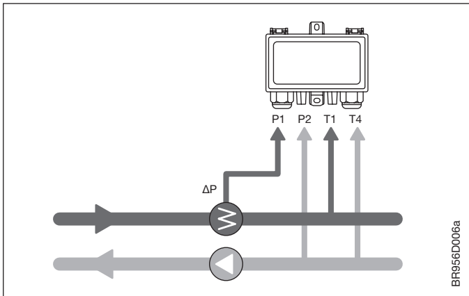
Fig 7 - Orientation of PTH
