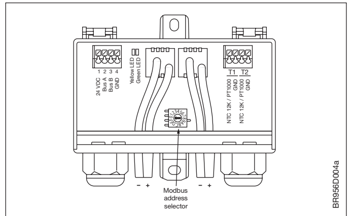
Fig. 6 - Modbus connections
