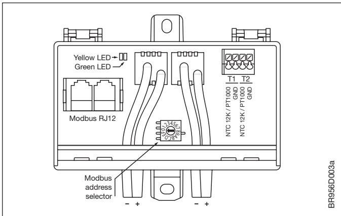
Fig. 5 - Example of configuration
