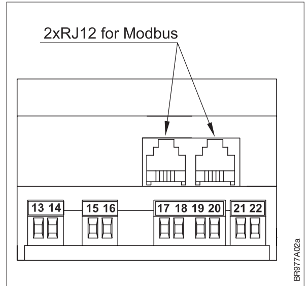
Fig. 2 - RJ12 ports for Modbus communication
